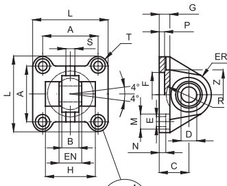
OUTLINE OF THE DIAMETER 32 Narrow rear eye with bearing DIN 648 K
